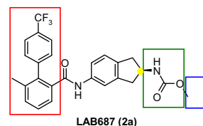
Figure 1. Structure of LAB687, a Hedgehog inhibitor screening hit.
